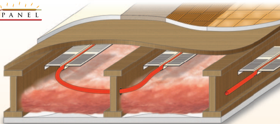
SUSPENDED CONVECTION FLOOR WITH Q-PANELS
